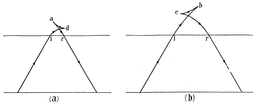
FIG. 8. Phase-rays of magneto-ionic components.
