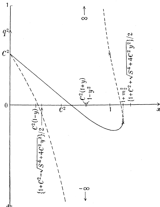
FIG. 21. Propagation in equatorial regions, y < 1 .
