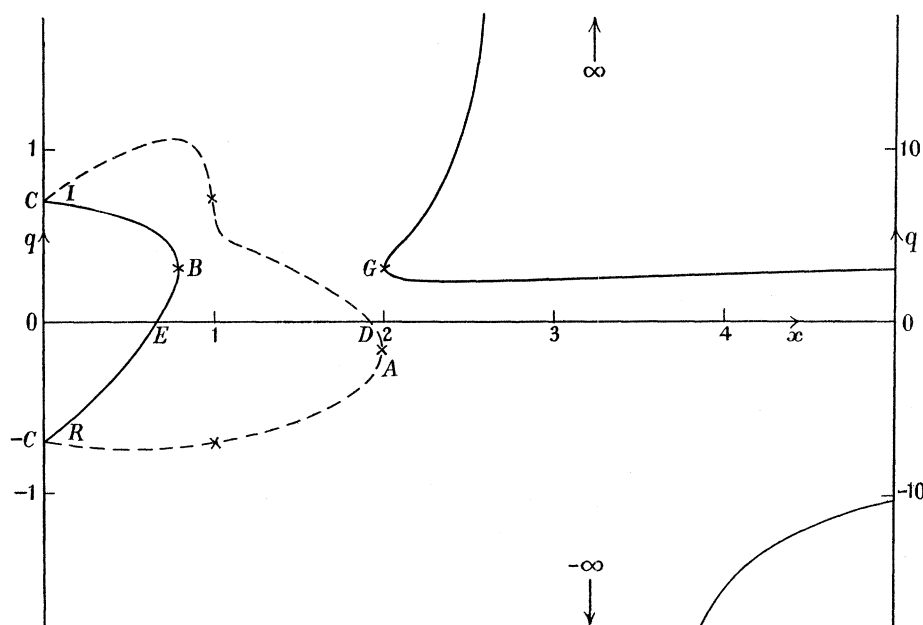
FIG. 16. q as a function of x , y > 1 .
