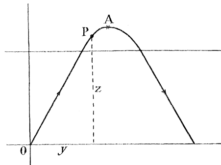
FIG. 10. The path of a wave-packet.
