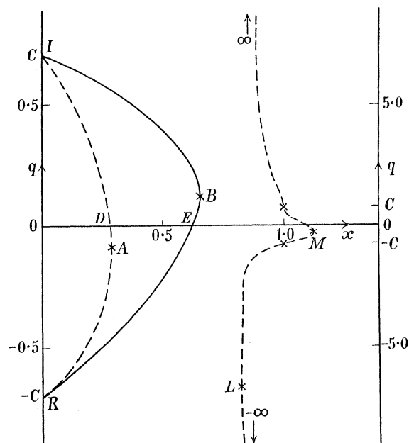
FIG. 15. q as a function of x, y < 1 .
