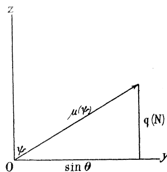
FIG. 4. Phase-propagation.
